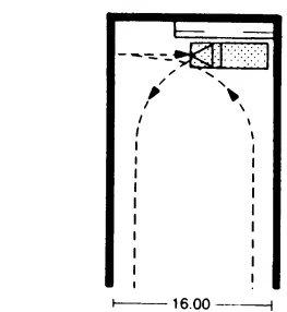
⑧ Turning in restricted areas
